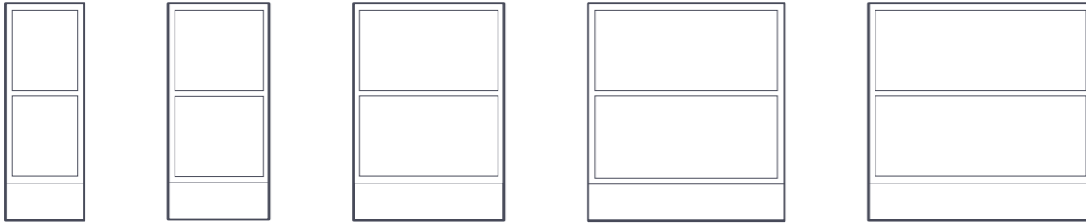
BH3/9 876X316X372 BH4/9 876X410X372 BH6/9 876X613X372 BH8/9 876X800X372 BH9/9 876X910X372
