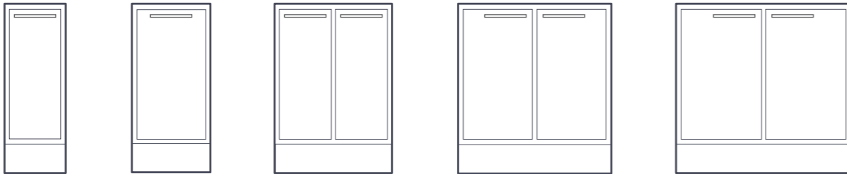
BD3/9 876X316X372 BD4/9 876X410X372 BD6/9 876X613X372 BD8/9 876X800X372 BD9/9 876X910X372
