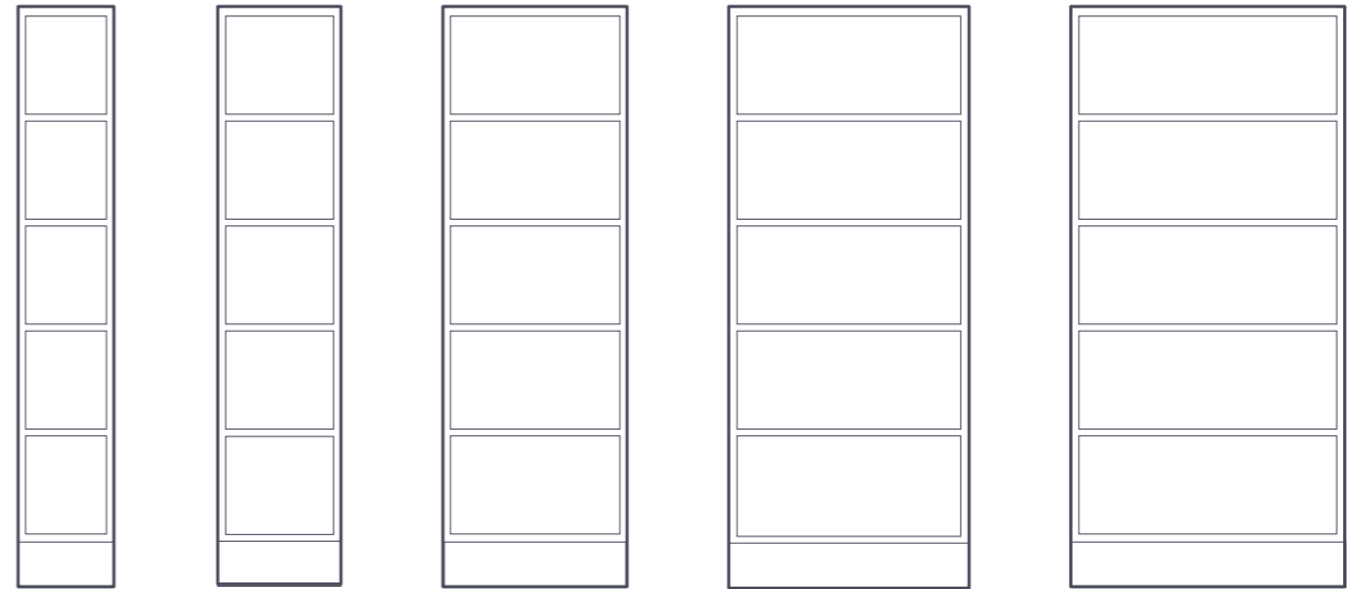
BH3/19 1932X316X372 BH4/19 1932X410X372 BH6/19 1932X613X372 BH8/19 1932X800X372 BH9/19 1932X910X372
