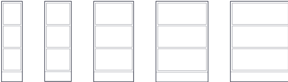
BH3/12 1228X316X372 BH4/12 1228X410X372 BH6/12 1228X613X372 BH8/12 1228X800X372 BH9/12 1228X910X372
