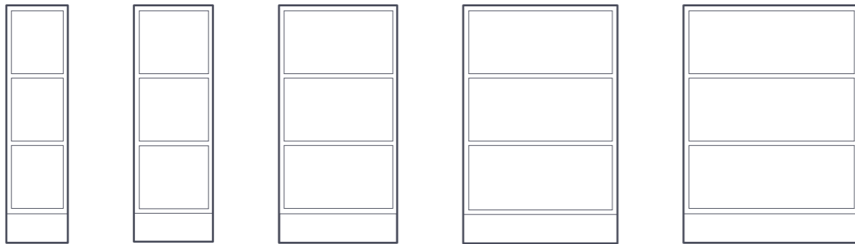
DH3/12 1228X316X580 DH4/12 1228X410X580 DH6/12 1228X613X580 DH8/12 1228X800X580 DH9/12 1228X910X580
