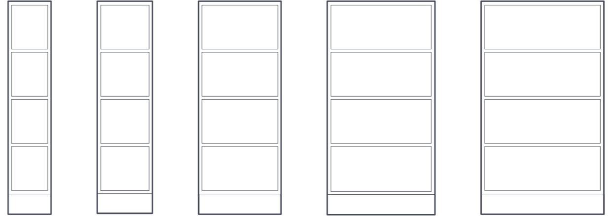
BH3/15 1580X316X372 BH4/15 1580X410X372 BH6/15 1580X613X372 BH8/15 1580X800X372 BH9/15 1580X910X372
