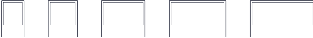
BH3/5 524X316X372 BH4/5 524X410X372 BH6/5 524X613X372 BH8/5 524X800X372 BH9/5 524X910X372
