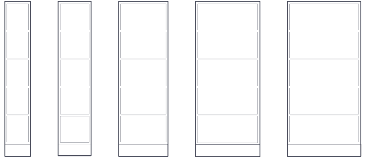
DH3/19 1932X316X580 DH4/19 1932X410X580 DH6/19 1932X613X580 DH8/19 1932X800X580 DH9/19 1932X910X580
