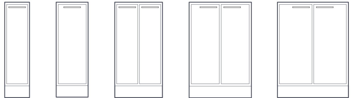
DD3/12 1228X316X580 DD4/12 1228X410X580 DD6/12 1228X613X580 DD8/12 1228X800X580 DD9/12 1228X910X580
