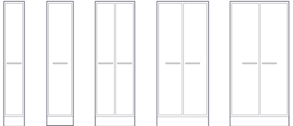
BD3/19 1932X316X372 BD4/19 1932X410X372 BD6/19 1932X613X372 BD8/19 1932X800X372 BD9/19 1932X910X372
