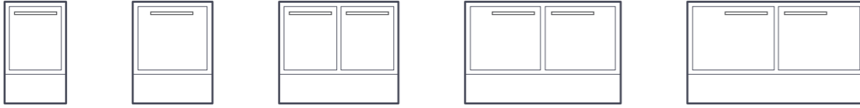
BD3/5 524X316X372 BD4/5 524X410X372 BD6/5 524X613X372 BD8/5 524X800X372 BD9/5 524X910X372
