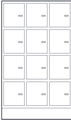
SF9/15 1580X910X372
