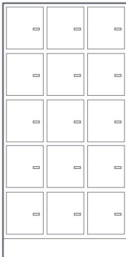
SF9/19 1932X910X372
