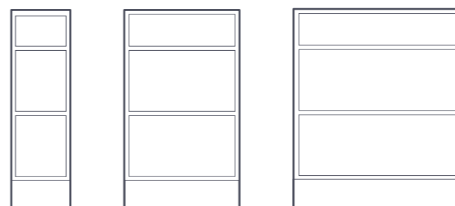
HH3/10 1068X316X580 HH6/10 1068X613X580 HH6/10 1068X910X580
