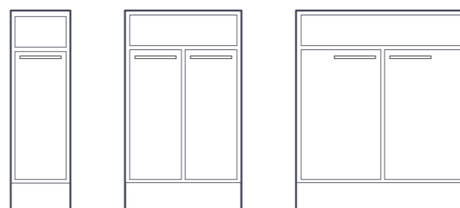
HD3/10 1068X316X580 HD6/10 1068X613X580 HD9/10 1068X910X580
