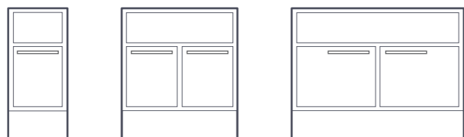
LD3/7 716X316X580 LD6/7 716X613X580 LD9/7 716X910X580
